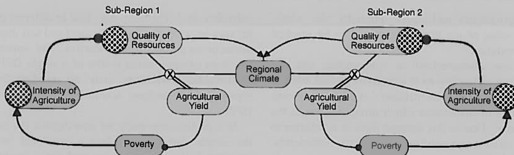
Fig. 13. Enhancement of the simple Sahel-HFP introducing two sub-regions coupled by a non-local landcover-climate interaction (for the definition of relations see Appendix).
