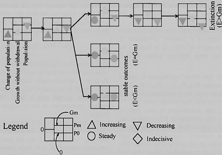
Fig. 8. Qualitative behaviours of the simple didactic model for a general logistic growth of the population dynamics. Each rectangle describes one qualitative state of the system. The black arrows points to possible successor states. Branches of the behaviour tree end either in stable equilibrium states or in "transition states" where the trajectory leaves the definition space of the model. For detailed explanation and discussion see text.
