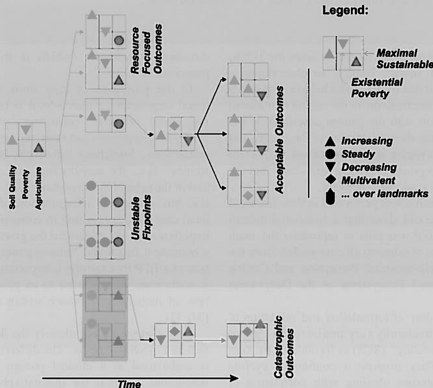
Fig. 12. "Behaviour tree" for the original Sahel HFP of causes and effects. Boxes and arrows indicate the qualitative states as explained by the legend on the right hand side. Time runs from left to right. Note that in some cases more than one successor is possible, e.g., for the initial state on the QSIM identifies seven possible successor states from the model.
