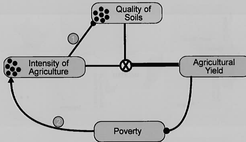
Fig. 9. Core mechanism of the original version of the SAHEL-SYNDROME. The symbols attached to the connecting lines uniquely encode qualitative relations as used within the concept of qualitative differential equations (QDEs). Their meaning is explained in the Appendix.
