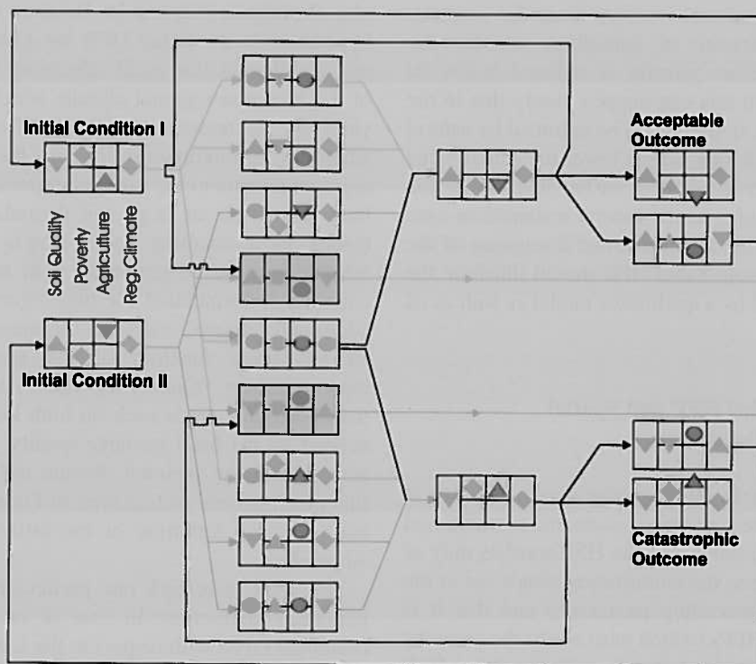
Fig. 14. Resulting behavior tree for the enhanced Sahel HFP (two sub-regions coupled by a non-local landcover-climate interaction) for one of the sub-regions. For a detailed legend see Figure 12.
