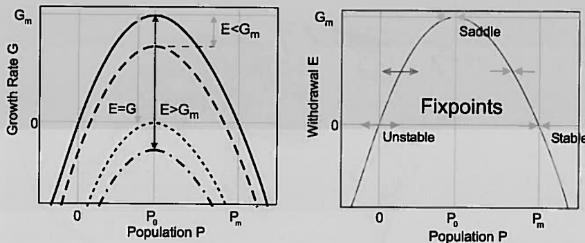
Fig. 7. Basic relation for the didactic model to explain the qualitative modelling approach. If subject to a constant withdrawal E , the U-shaped relation between the population P and the growth rate G gives rise to three different types of behaviour. Starting from the climax state P = P_m , the population either stabilises at a level beyond P_0 , if the withdrawal is less than G_m (dashed line) or right at P_0 if E = G_m (dotted line). In case of E > G_m , the population finally vanishes (dot-dashed line).
