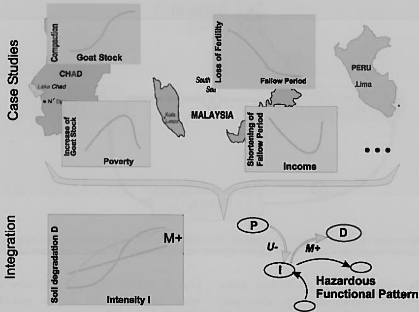
Fig. 10. Scheme of generalisation used to formulate a class of civilisation-nature interactions. Case studies might be used to specify the regionally valid relations between relevant variables. Abstracting these variables into more general concepts, e.g., Intensity or Soil Degradation, are then used to specify qualitative relations between the abstracted variables. In the example given the qualitative relations, indicated by the notions U- and M+ in the cause-effect scheme on the lower right hand side, contains the (hypothetical) situation in Chad as well as in Malaysia and possibly Peru.
