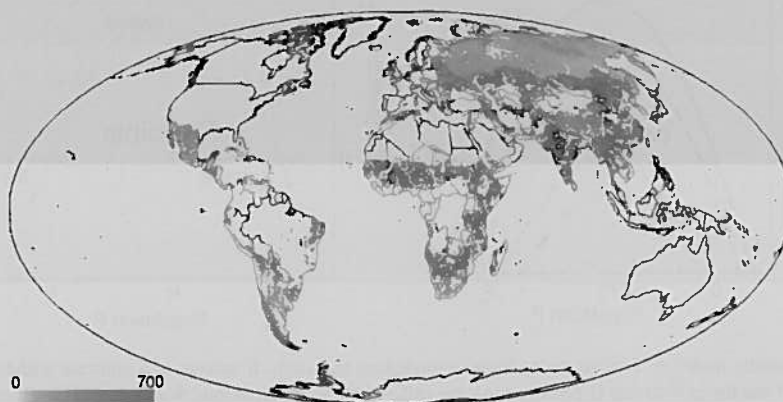
Fig. 6. Climate sensitivity of the disposition towards the SAHEL SYNDROME.
