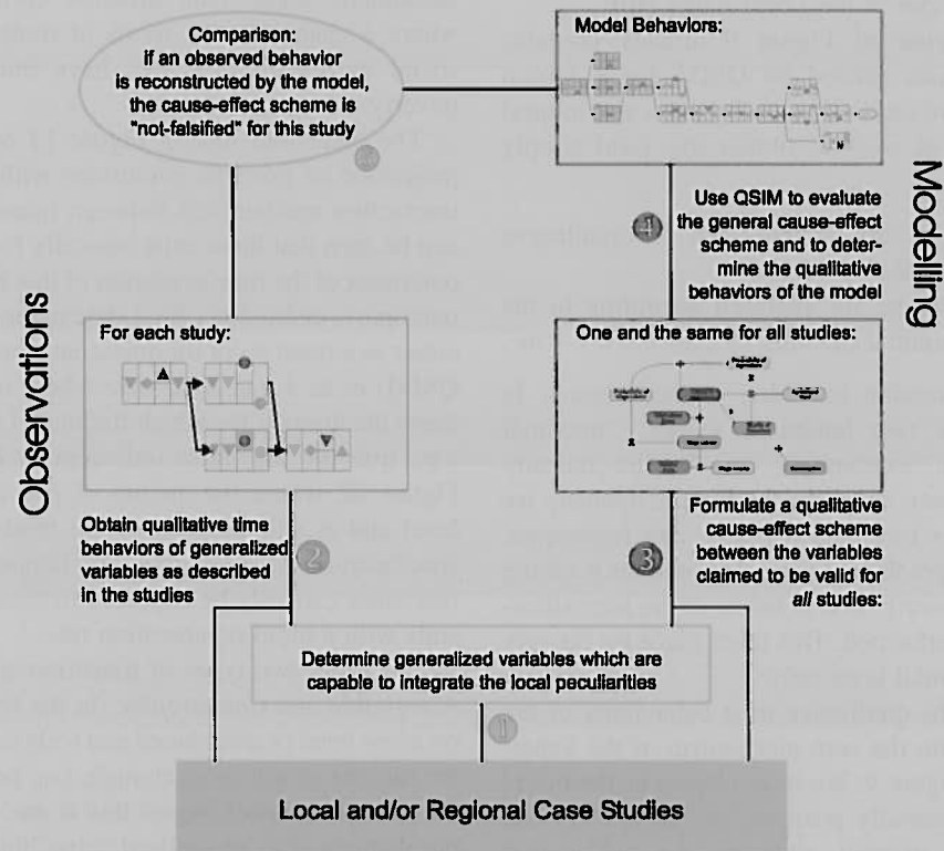
Fig. 11. General scheme of case study integration into a common class of causes and effects.
