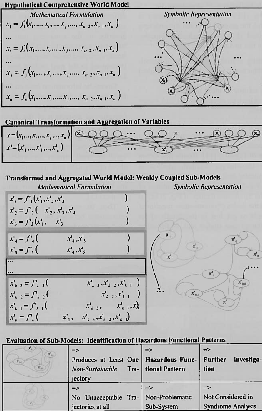
Fig. 1. Hypothesized process of the deduction of Hazardous Functional Patterns producing Syndromes as classes of non-sustainable time behaviours.
