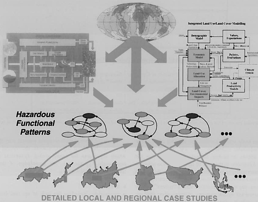
Fig. 2. Approaches for identifying of Hazardous Functional Patterns (“ intermediate functional scale ”): general functional knowledge and problematic global developments (top-down) versus generalisation of detailed case studies (bottom-up).
